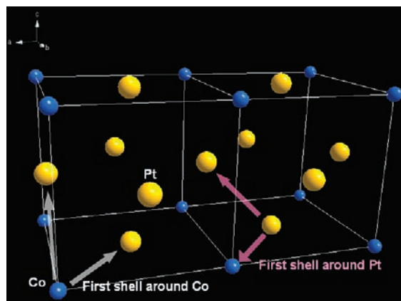
Figure 7. Face-centered cubic structure of CoPt 3 and first shell scattering modes of Co/Pt atoms.
